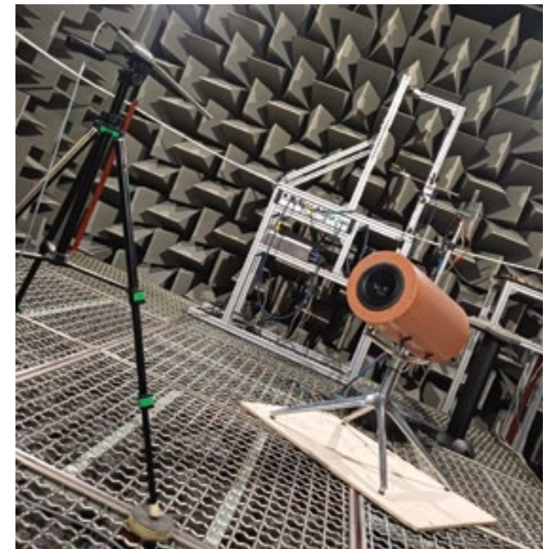
DRUM D260 BT - 6,5 inch coaxial, rear-facing bass reflex, active class D amplified Bluetooth speaker
